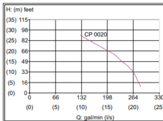
H: Head feet (m) Q: Flow imp gal/min (l/s)
